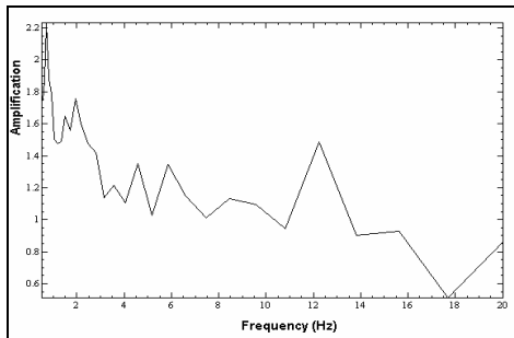
Figure 9. HVSR inside to Roman Reservoirs.
