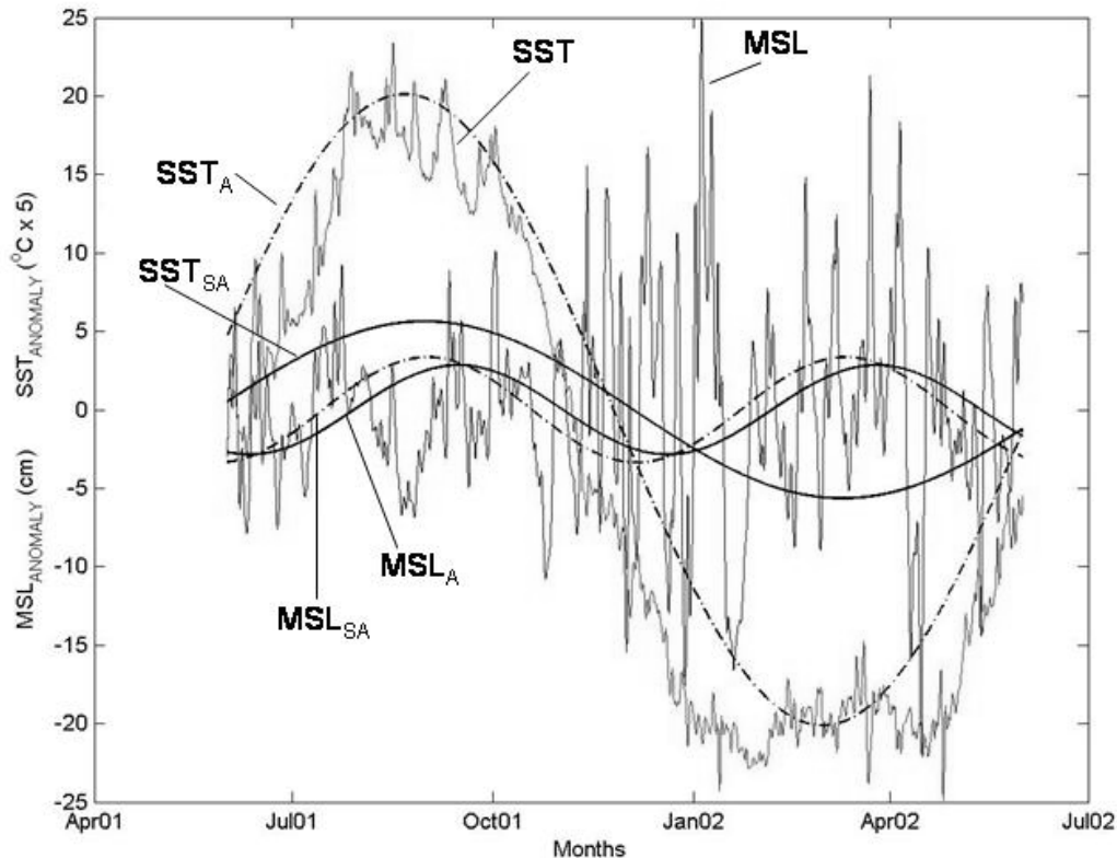
Figure 4. Taxiarhis station anomalies of MSL and SST with the correspondent annual ( MSL_A , SST_A ) and semiannual harmonics ( MSL_{SA} , SST_{SA} ).
