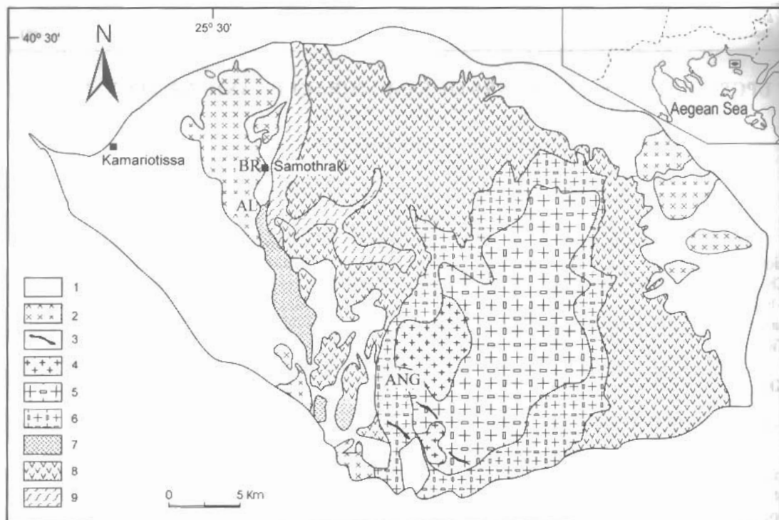
Fig. 1. Schematic geological map of the Samothraki island according to Christofides et al. (2000). 1:Tertiary-Quaternary sedimentary rocks, 2:Tertiary volcanics, 3:Micro-granite, 4: Biotite-granite, 5:Porphyritic quartz-monzonite to granite, 6:Porphyritic micro-quartz-monzonite to micro-granite, 7:Gabbrodiorite, 8:Ophiolites, 9:Basement rocks. BR = Brehos, AL = Alonia, ANG = Anginaros.
