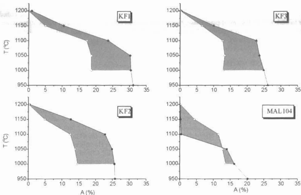
Fig. 2. Effect of temperature ( T^{\circ}\text{C} ) on water absorption ( A\% ) of the four specimens studied from Samothraki igneous rocks. Open symbols = treated material, closed symbols = non-treated material.
