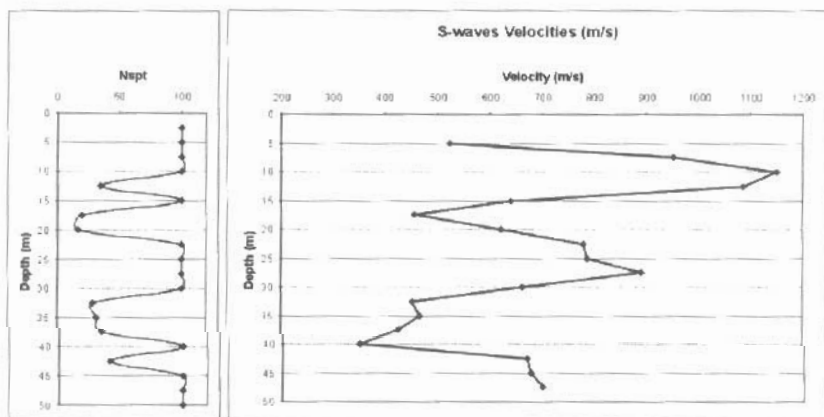
* Nspt value 100 is representative of refusal Ηφιακή Βιβλιοθήκη "Θεόφραστος" - Τμήμα Γεωλογίας, Α.Π.Θ. Figure 4: Nspt and S-wave velocity comparison
