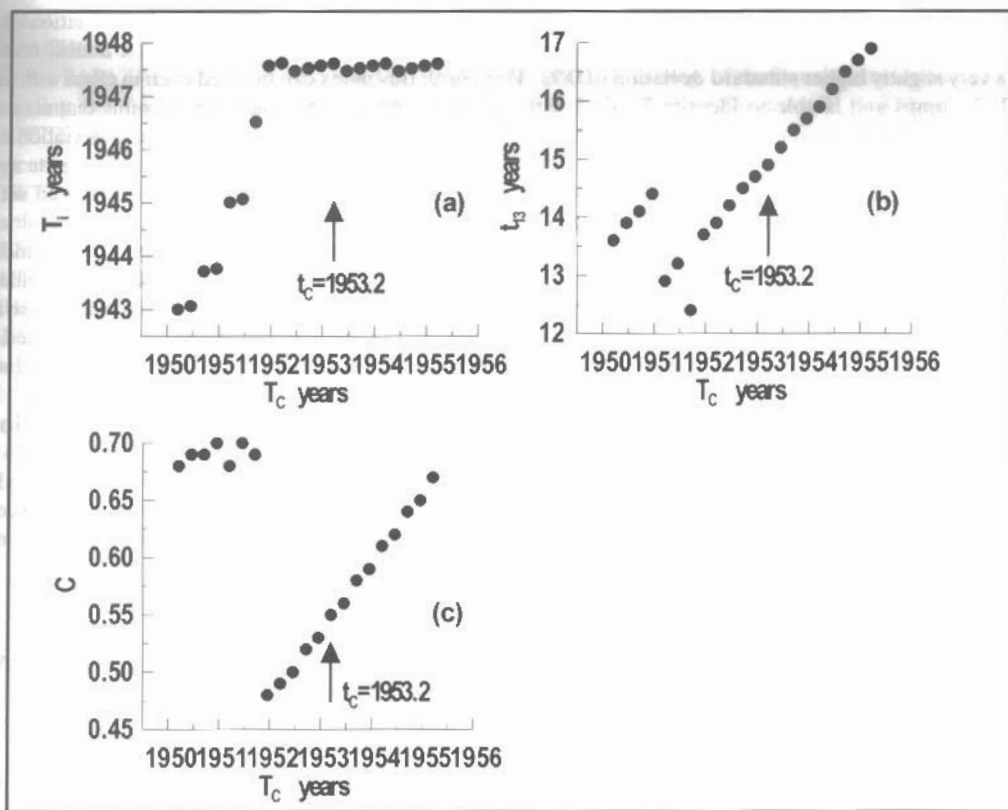
Figure 1) shows an example of a T_i - T_c , a t_{13} - T_c and a C - T_c graph for the 13.08.1953, M=7.4 , 40.0^\circ N , 27.5^\circ E earthquake, where the origin time, t_o of this shock is also indicated by an arrow. It is observed that an abrupt increase of T_i and decrease of t_{13} and C occur for T_c = T_o = 1951.71 . It corresponds to T_i = 1947.57 which is the time when this precursory phenomenon (seismic excitation) took place. We should point out that C does not decrease (as expected) as we get closer to the mainshock time, T_o , because we allow T_c to vary and take several values that are "candidates" for the "real" mainshock occurrence times, t_o .
