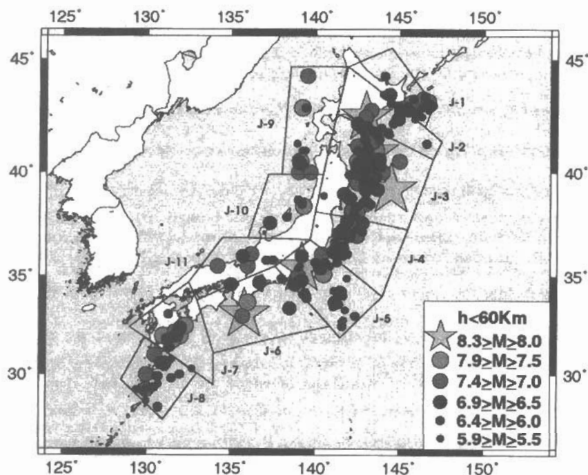
Fig.1. Geographical distribution of the epicenters of the shallow earthquakes and the examined seismogenic source (Papazachos et al. (1997), Ελληνική Βιβλιοθήκη "Θεόφραστος" Δι Τμήμα Πεωλογίας Α.Π.Θ. , 1997).
