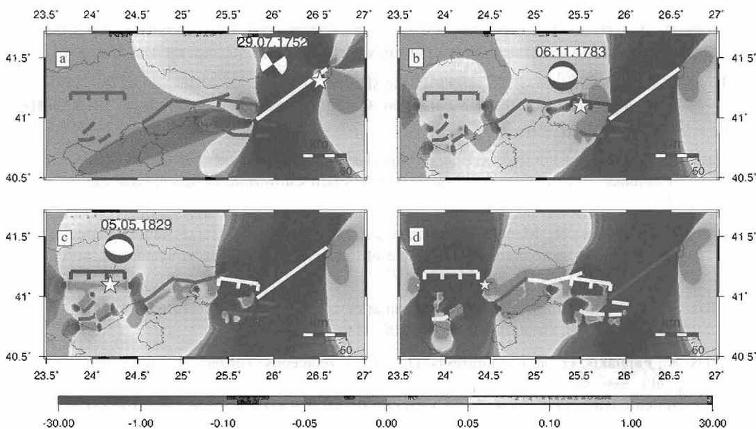
Figure 4 - Stress evolution in Eastern Macedonia and Thrace since 1752. Faults in black represent the target faults according to which the stress changes have been calculated, faults in white represent faults that have slipped in strong earthquakes, and faults in gray are the active ones that still remain unruptured. Fault plane solutions are shown as lower hemisphere equal area projections and main shock epicenters are depicted by a star. A gray scale is used to present schematically the stress changes, measured in bars. (a) Co-seismic Coulomb stress changes associated with the 1752 event. (b) Stress evolution until just before the 1783 event calculated according to its fault plane solution. (c) \Delta CFF just before the 1829 main event. (d) State of stress in 2006 computed for the dip slip approximately east-west striking faults
