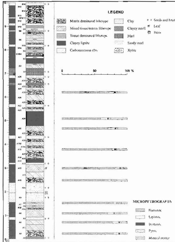
Figure 8 - Micro- and macropetrographical analysis of coal seams in studied area
