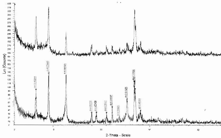
Figure 4 - X ray diffraction diagrams of A9a sample, before and after heating up to 550 °C
