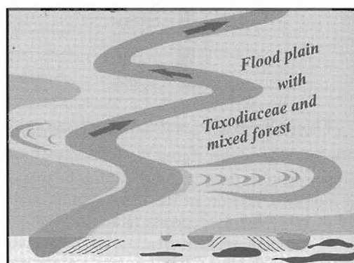
Figure 10 - Paleoecological reconstruction of the general area
