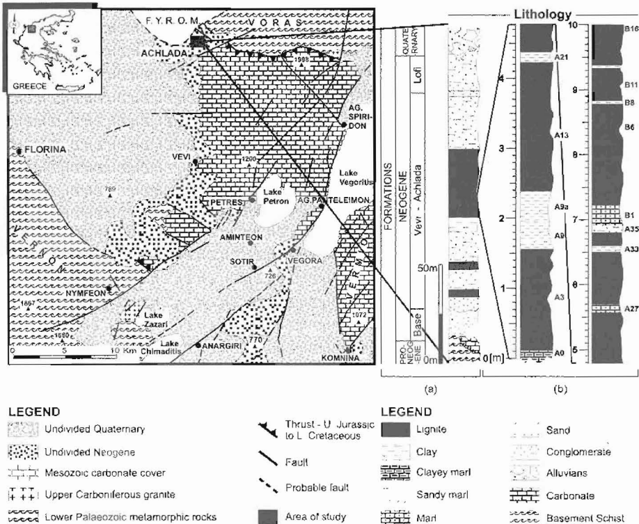
Figure 1 - Geological map of the Florina basin with the location and the generalized lithological column (a) of the studied area (after Pavliades and Mountrakis 1987). (b) lithological column of Achlada lignite deposits
