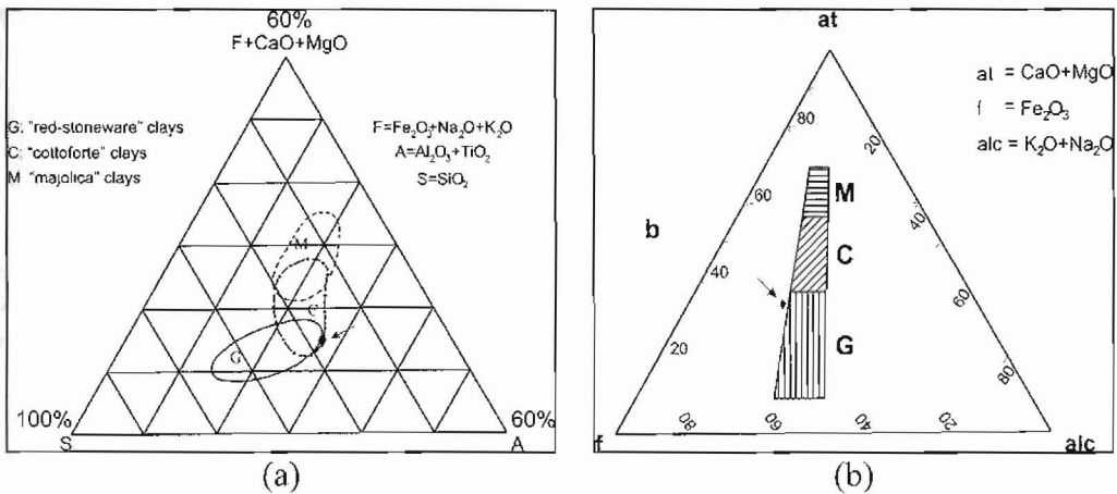
Figure 11 - (a) Ternary diagram \text{SiO}_2/\text{Al}_2\text{O}_3+\text{TiO}_2/\text{Fe}_2\text{O}_3+\text{MgO}+\text{CaO}+\text{K}_2\text{O}+\text{Na}_2\text{O} , (b) Ternary diagram \text{Fe}_2\text{O}/\text{MgO}+\text{CaO}/\text{K}_2\text{O}+\text{Na}_2\text{O}
