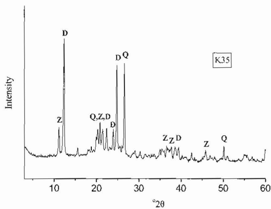
Figure 3b - XRD pattern of the bulk sample K35 (D: dickite, Z: Zunyite, Q: quartz)
