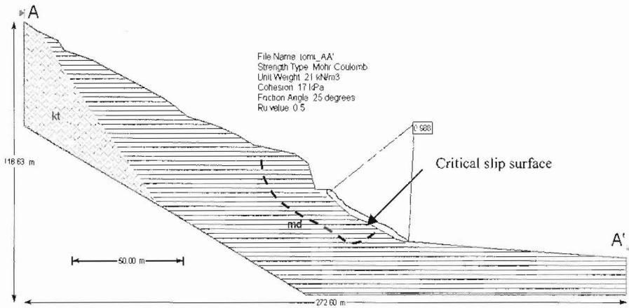
Figure 6 - Cross-section AA'
