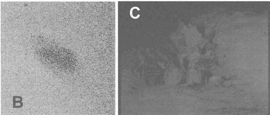
Figure 5 - A: Section of 3.5 kHz subbottom profile from the Oreoi straits, North Evia. The profile shows the 6-meters thick, acoustically transparent, Holocene sedimentary drape overlying unconformably Pre-Holocene deposits. B: Extract from a side scan sonar record showing a strongly backscattering target from the area where the profile of Fig. 5A was acquired. C: Photograph taken by ROV Super Achilles during the visual inspection of the previous target. The target was proved to be a concentration of living bivalves and various shells on the seafloor
