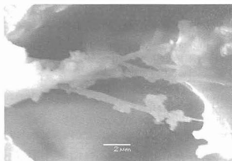
Figure 9 - Tiny crystals of halite
