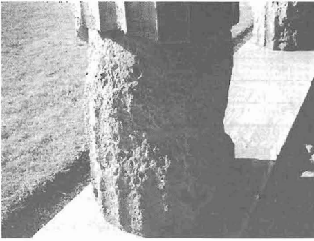
Figure 12 - Honeycomb decay of bottom column piece of type I sandstone, and shape alteration
