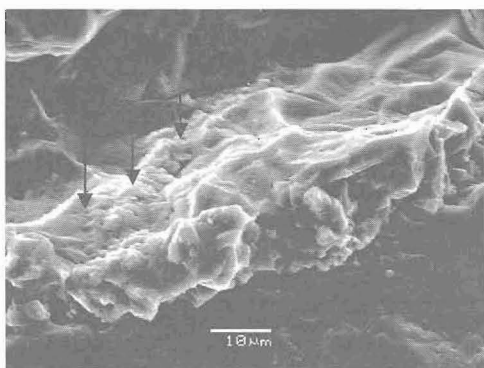
Figure 11 - Dissolution patterns and pits (arrow) on calcite cement, due to solution attack
