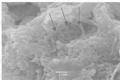
Figure 8 - Micromorphisms development in pores
