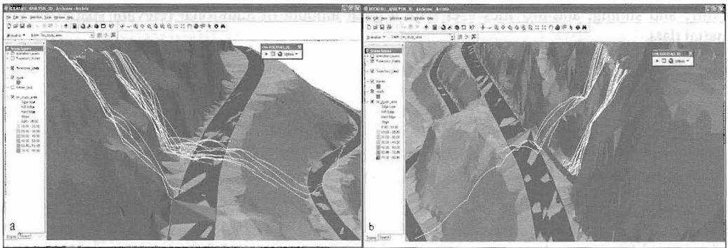
Figure 4 - a. Rockfall simulations in the case where a barrier is not used. b. Rockfall simulations in the case where a barrier is evaluated as a countermeasure
