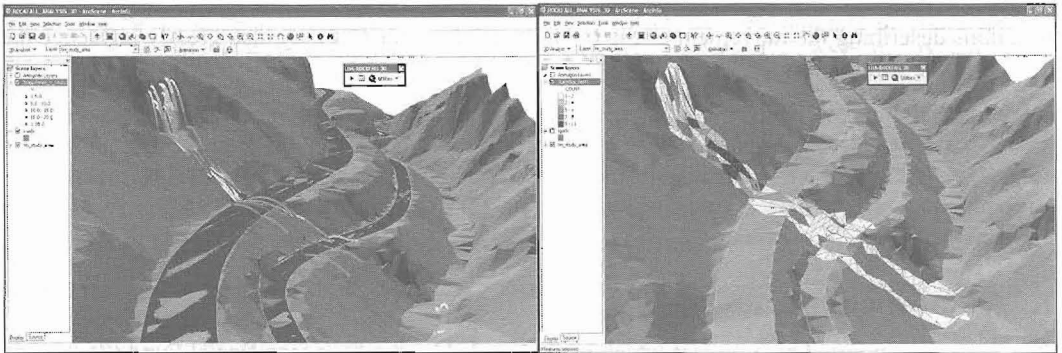
Figure 5 - a. The symbology of rockfalls based on the velocity rock boulders have along their trajectory. b. The subarea subjected to the simulated rockfalls. The triangles are symbolized based on the number of rockfalls traversing each triangle
