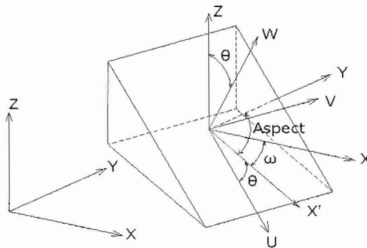
Figure 1 – The two reference coordinate Cartesian systems of the rockfall simulation model: the “Global” coordinate system (XYZ) and the “Local” coordinate system (UVW), and the relationship between them (Charalambous 2006)
