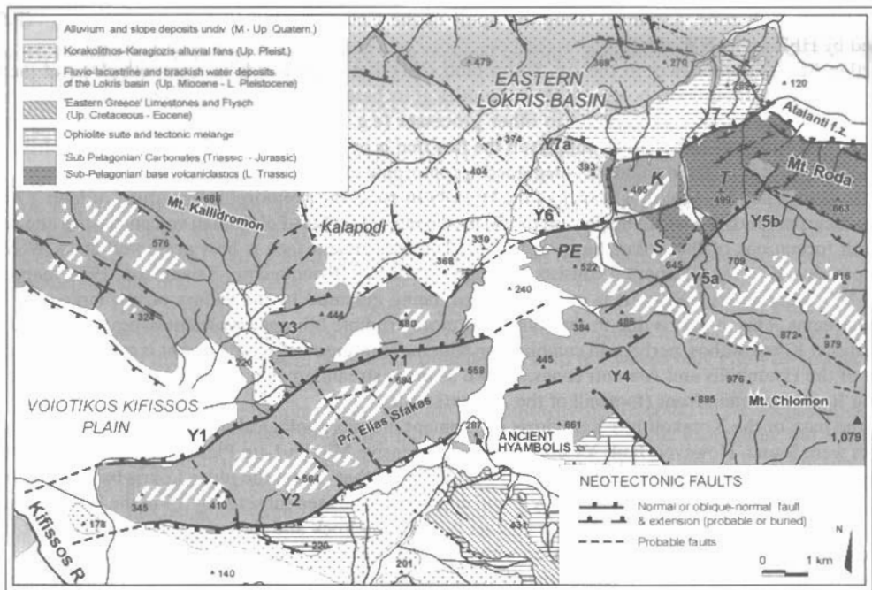
Fig. 2. Geological-neotectonic sketch map of the area crossed by the HFZ. Geology after Maratos et al. (1965, 1967), Sideris (1986), Kranis (1999) and Palyvos (2001). Faults from Kranis (1999) and Palyvos (2001). Thick white lines indicate remains of the Chlomon Miocene relief.
