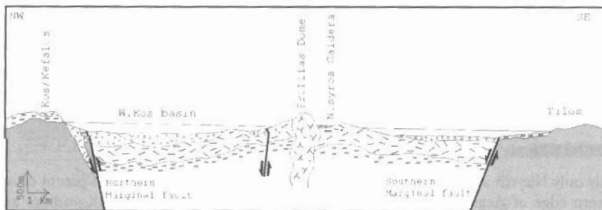
Fig 2a: Schematic tectonic profile through Kos-Nisyros-Tilos.
