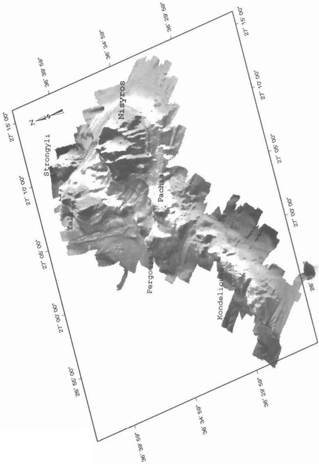
Fig 4: Perspective image of Nisyros and neighbouring volcanic islets. View from SW.
