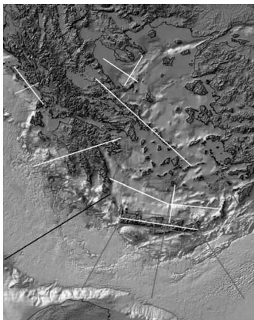
Fig. 1: Location of seismic lines recorded in 1971-1974 and 1982-1984 in white. Red are 2D-lines mapped in 1994 to 2008. In black is a composite line that has been obtained from 2 ships experiments and published by De Voogd et al. in 1992.
