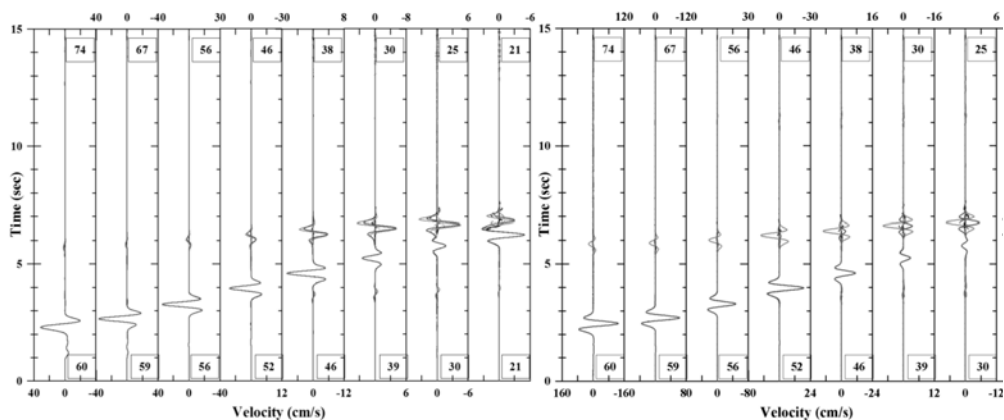
Fig. 3: Longitudinal components of FD and NRB synthetics for model A and direct P waves incidence (left) and for model B and direct S waves incidence (right). Coloring and numbering is described in the 3 rd paragraph of current page.
