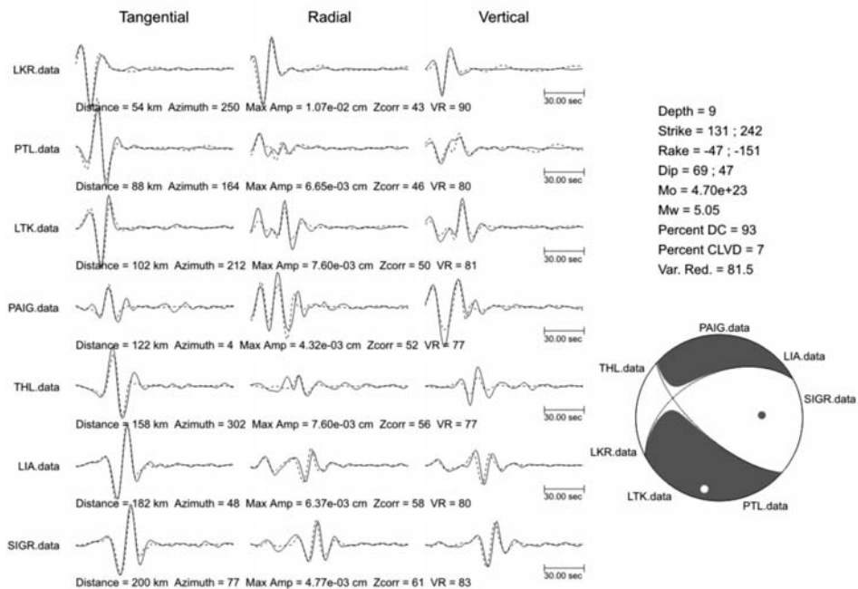
Fig. 1: Moment tensor solution for the 14 October 2008, GMT 02:06 earthquake (No 1 in Table 1). Used stations provide the best azimuthal coverage of the epicentre without over-weighting any azimuth. For each station waveform fit between observed (continuous lines) and synthetic (dashed lines) vertical, tangential and radial components are shown (left). Solution parameters are summarized in the right part of the figure.
