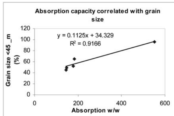
Fig. 5: The relation of the fineness at <45 \mu m passing grain size and the absorption capacity [ <0.3 mm fraction].
