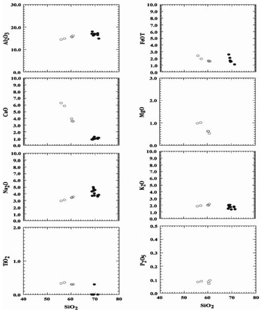
Fig. 6: Harker plots for the major elements, of the Xylokastro volcanic ash bulk samples and glass showing the variations in their composition. (The empty cycles represent the bulk sample compositions and the full cycles the glass microprobe analyses).
