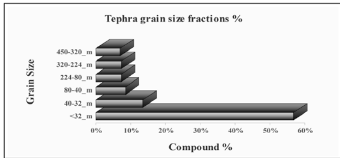
Fig. 5: Grain size distribution in the Xylokastro volcanic ash bed.
