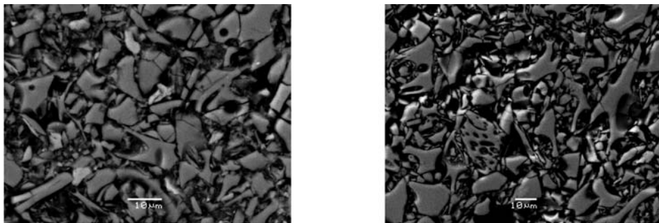
Fig 8a: SEM images of the Xylokastro ash bed: Glass shards. Note the fineness of the particles [size <20μm].
