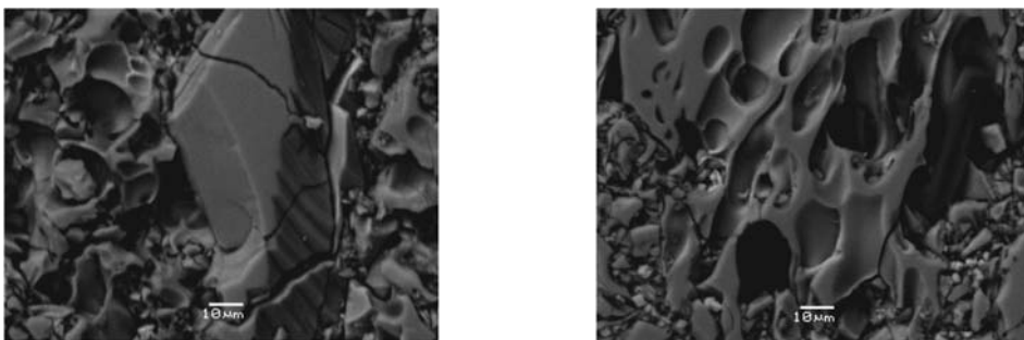
Fig. 8b: SEM images of the Xylokastro ash bed: Pumice and feldspar fragments [left image]. The particle size of both components is higher than that of the glass shards.
