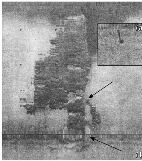
Fig. 19. Side scan sonar sonographs showing (a) a high relief target which represents an iron anchor and (b) an amphora concentration which represents an ancient shipwreck.
