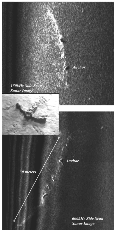
Fig.1. 150 kHz and 600 kHz side scan sonar images showing an ancient shipwreck lying on the sea-floor (water depth 750 m) and the iron anchor resting atop the remains of the hull of the shipwreck. Inset digital photo showing iron anchor resting on the sea-floor (Phaneuf, Ciavola, Papatheodorou and Ferentinos, 2002).
