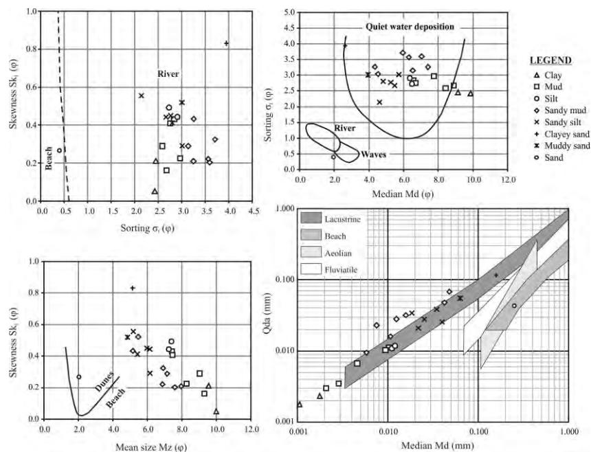
Figure 3 – Scatter diagrams of the statistical particle-size parameters (Stewart, 1958; Buller and McManus, 1972; Amaral and Pryor, 1977; Friedman, 1979) showing the origin of the sediments and the deposition environment.
