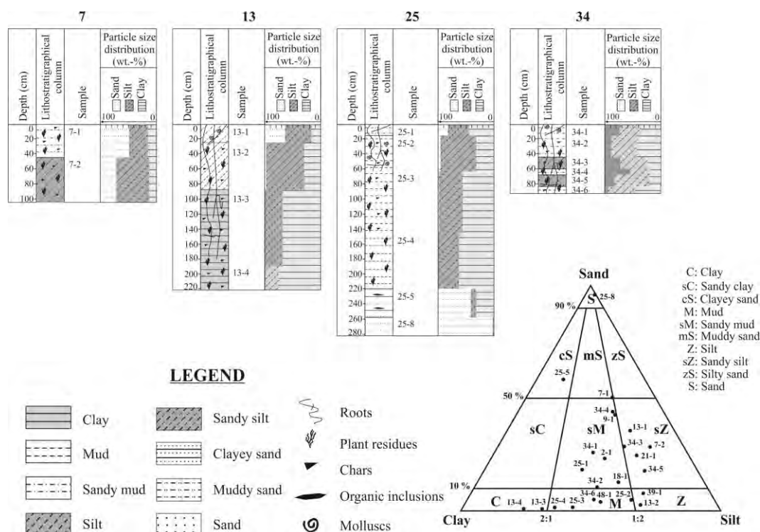
Figure 2 - Detailed lithostratigraphical columns showing the vertical particle size distribution (wt.%) of the soil pits and ternary diagram for the classification of all the samples according to Folk (1954).
