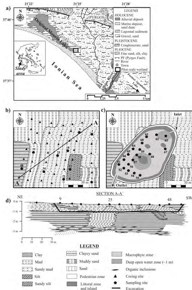
Figure 1 - a) Simplified geological map of the Pyrgos area (after Chatziapostolou et al., 2008), b) Geological map of the pilot-scale wetland before its construction, c) Sketch-map of the pilot-scale wetland and the sampling sites, after re-flooding with rainwater, d) Cross section AA'.
