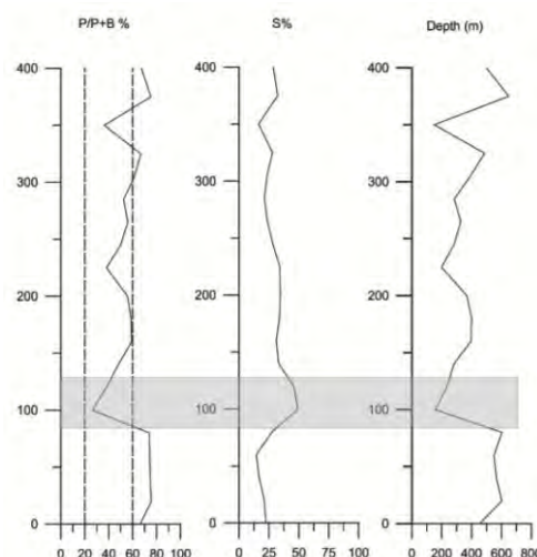
Figure 3 - Planktonic/Benthic ratio together with well-established redox front dwelling taxa and palaeobathymetric curve.
