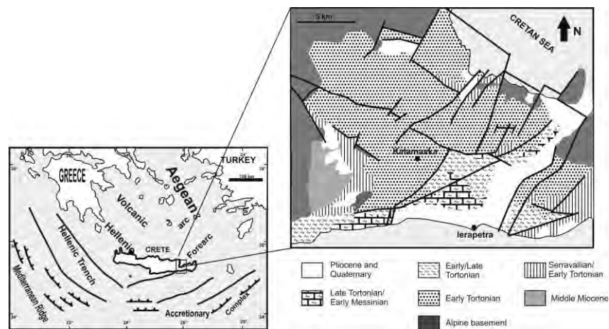
Figure 1 - Geological Sketch map of the Ierapetra Basin (modified from Fortuin 1977, 1978).
