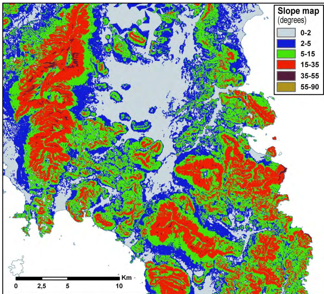
Figure 2 - Slope map of the study area.
