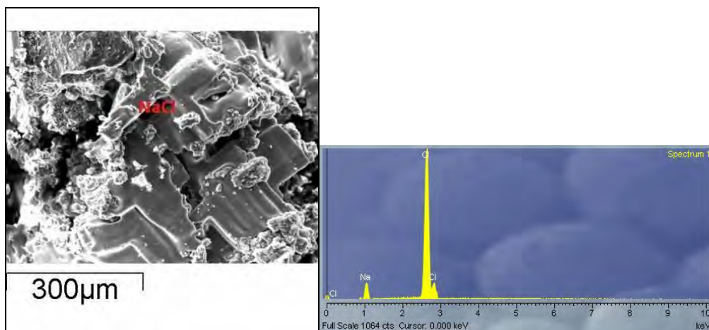
Figure 10 - SEM micrograph of the mortar C and EDS analysis of halite.
