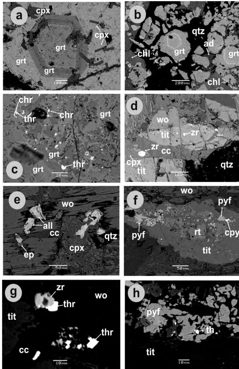
Figure 2 - Microphotographs demonstrating mineralogical assemblages of the Kimmeria skarn (SEM-BSE images). (a) Idiomorphic zoned garnet crystal (gnt) intergrown with clinopyroxene (cpx). (b) Garnets (gnt) replaced by retrograde quartz (qtz), chlorite (chl) and adularia (ad). (c) Chromite (chr) and uranothorianite (thr) included in garnet (gnt). (d) Titanite (tit) including zircon (zr) replaced by calcite (cc). Wollastonite (wo) and clinopyroxene (cpx) are also present. (e) Allanite (all), epidote (ep), quartz (qtz) and calcite (cc) postdate wollastonite (wo) and clinopyroxene (cpx). (f) Titanite (tit) crystal with inclusions of pyrophanite
