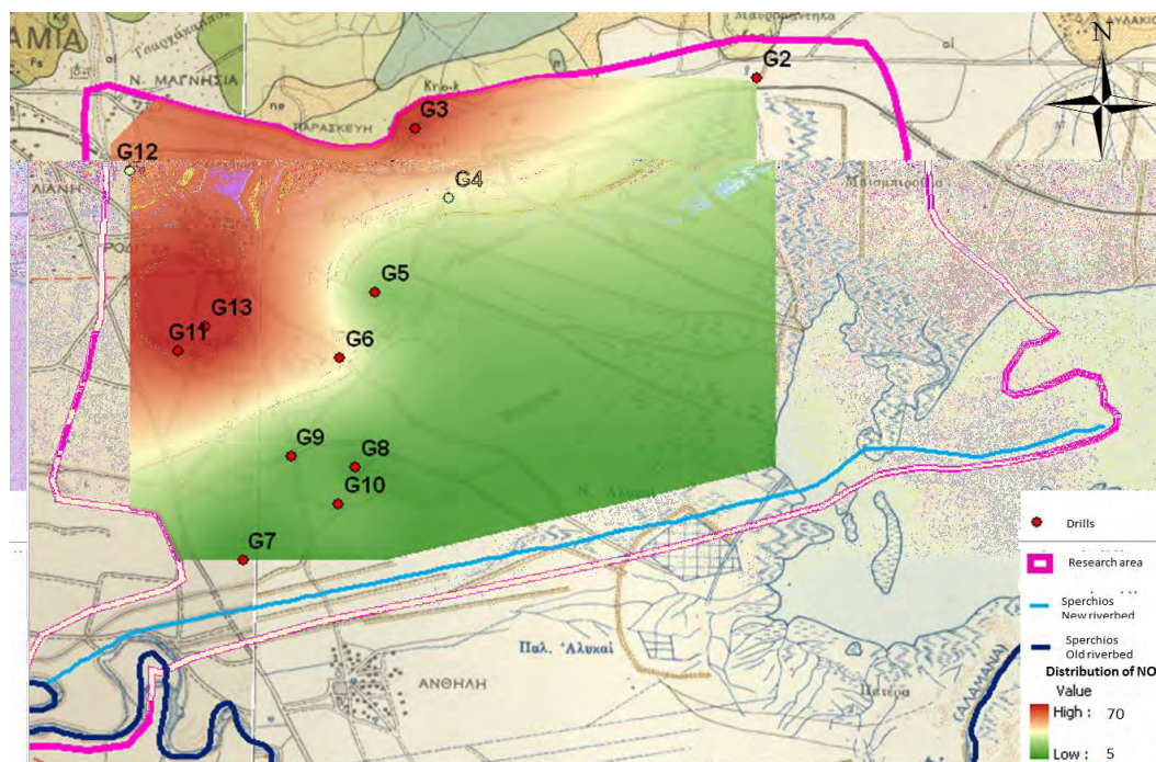
Figure 4 - Distribution map of \text{NO}_3^- in groundwater.
