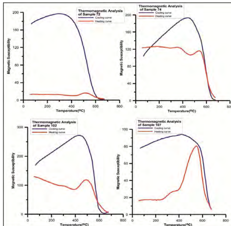
Figure 5 - Thermomagnetic curves of samples showing magnetic behavior.
