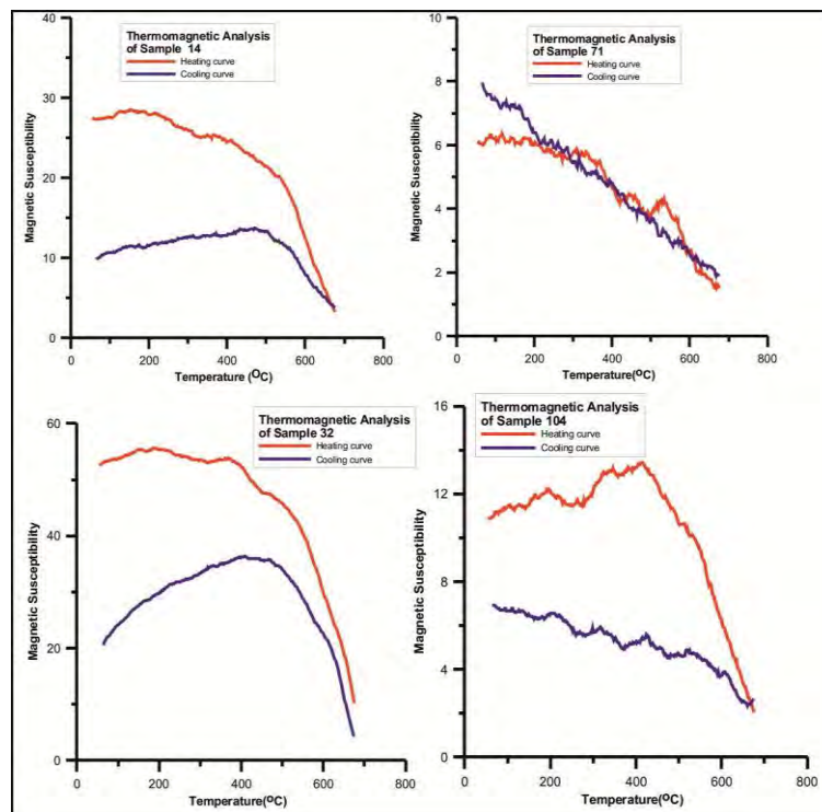
Figure 6- Thermomagnetic curves of samples showing paramagnetic behavior.
