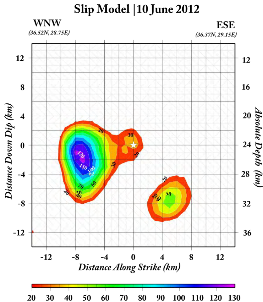
Figure 5. Slip model for the event of 10 June 2012 M_w 6.0 event obtained from the inversion of broad band waveforms, for the N115^\circ E trending fault plane, adopting a rupture velocity of 2.9 km/s, found from a standard grid search of the parameter space. One main slip patch is calculated where the peak slip value (~125 cm) was observed, with approximate dimensions 5 \times 5 km 2 . The asterisk denotes the hypocentre location, which lies at an absolute depth of 24 km. Note that the locus of slip is concentrated ~4 km to the NW of the hypocenter, and if directivity is present, it should be in that direction. A second slip patch is also observed, which is deeper than the previous and less pronounced, but which was a stable feature in all test inversions and fits the long lapse time in the data.
