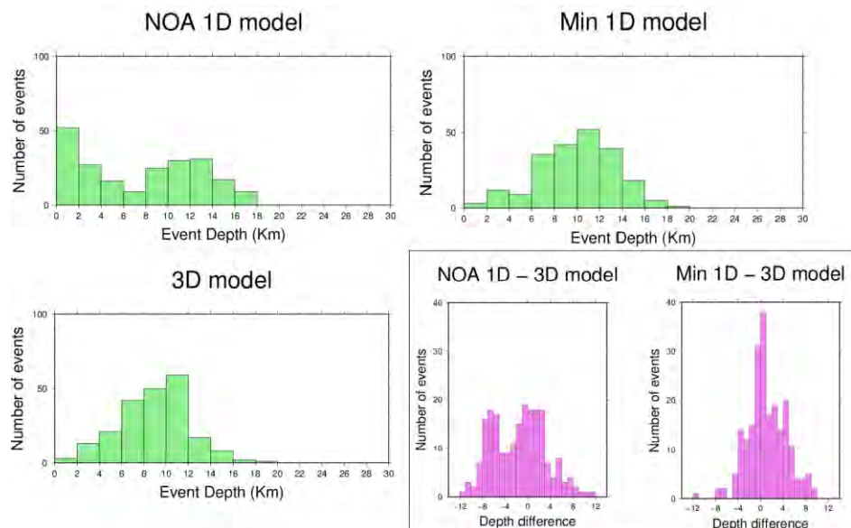
Figure 8 – Depth distribution of the events for the NOA 1D model (top left), the minimum 1D model (top right) and the 3D model (bottom left). Depth differences for the located earthquakes, between the 3D and the 1D models are also presented in this figure (bottom right).
