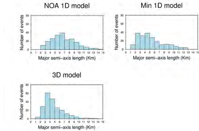
Figure 5 – Distribution of the major ellipsoid semi-axes for the NOA 1D model (top left), the minimum 1D model (top right) and the 3D model (bottom left).
