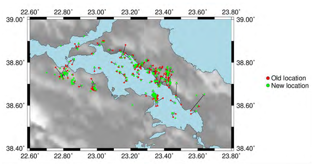
Figure 7 – Locations obtained by the minimum 1D model (red) and the 3D model (green). Only the events located with azimuthal gap lower than 180^\circ are shown.
