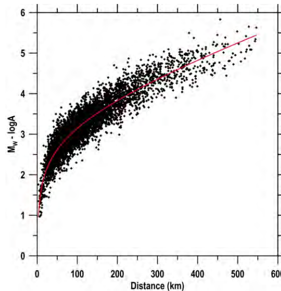
Figure 4- Calibration function for shallow ( h < 40\text{km} ) earthquakes after applying the stations' corrections listed on table 1. The line represents the best fitting the data curve.
