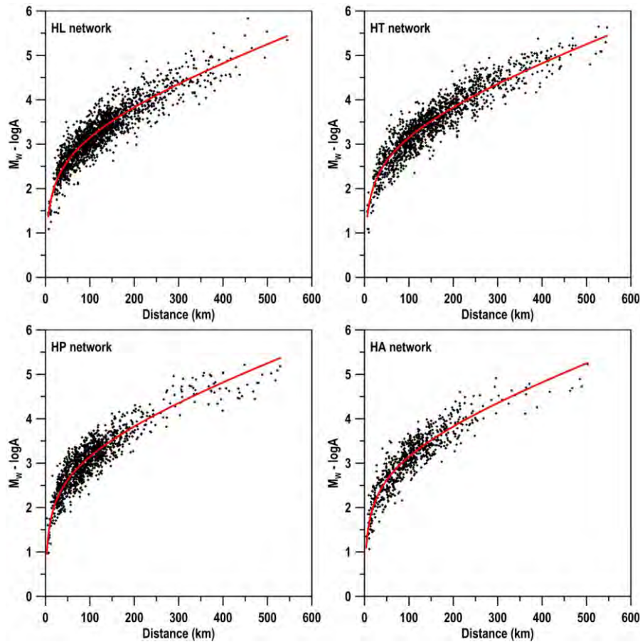
Figure 5 - Plot of M - \log A versus hypocentral distance for the stations of each one of the four participating networks (the lines represent the final calibration function defined in the present work).
