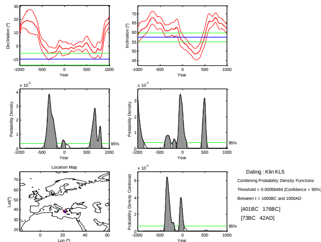
Figure 6 - Archaeomagnetic dating results for a) KL3 and b) KL5 kilns. Dating intervals have been calculated at 95% of probability using the matlab archaeo_dating tool (Pavón-Carrasco et al., 2011).
