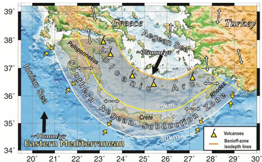
Figure 1 – Geotectonic setting of the broader Southern Aegean subduction area. Isodepths of the Benioff-zone, as well as the volcanic arc are shown. Single solid and double open vectors depict the plate motions and local stress field in the area, respectively (modified from Papazachos et al. 1998, Karagianni et al., 2005).
