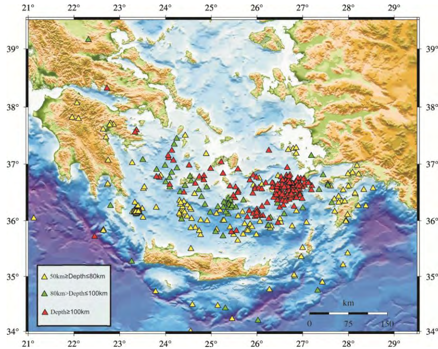
Figure 3 – Epicentral and depth distribution of all intermediate depth earthquakes employed for the Southern Aegean attenuation structure.
