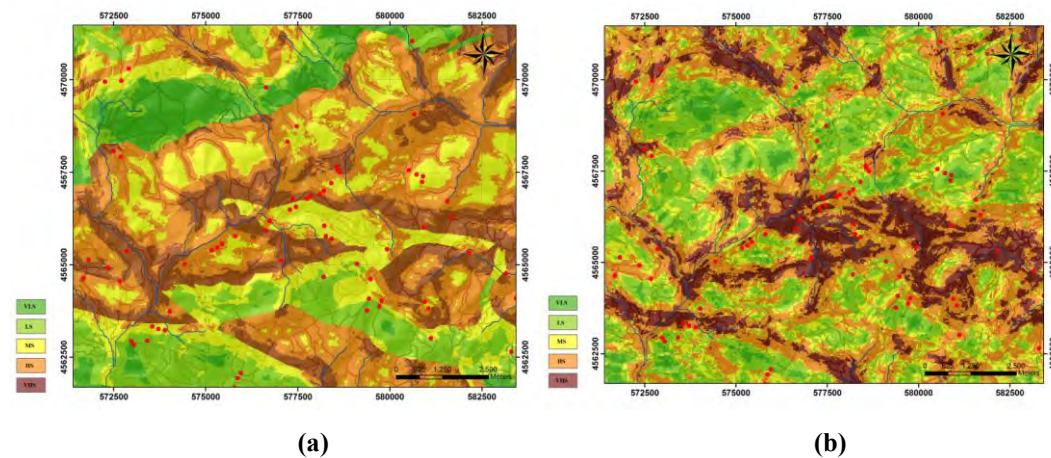
Figure 6 – The Landslide Susceptibility Maps: (a) AHP and (b) RES method.
