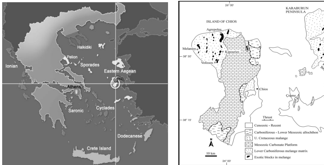
Figure 1 - Location of Chios Island (left); Simplified lithological map of Chios Island (right) (abstracted from Robertson & Ustaömer, 2009).
