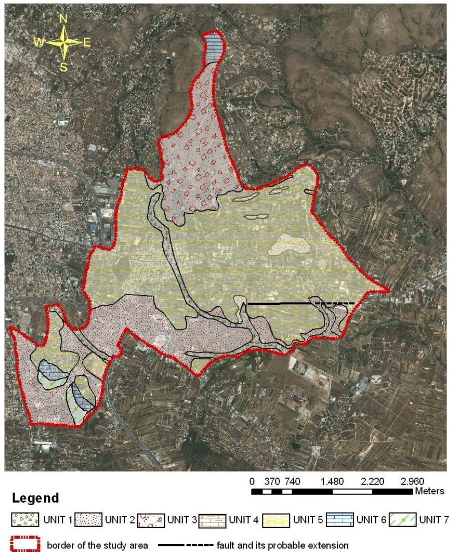
Figure 4 – Engineering geological map of Pallini prefecture.
