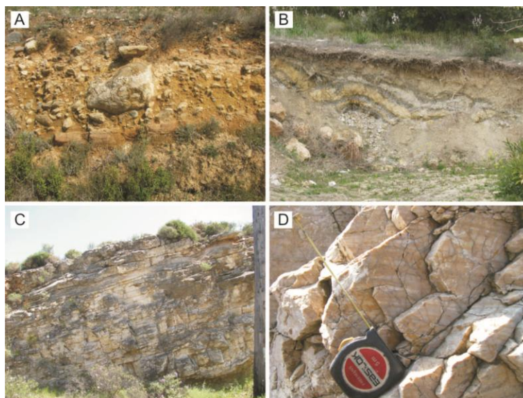
Figure 2 – (a) Mixed phase formations of fluviolacustrine origin, (b) Marls' slubbings, (c) intensively fractured travertine, (d) intensively fractured marbles.
