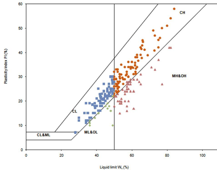
Figure 3 – Projection of the samples studied in the Casagrande plasticity chart.
