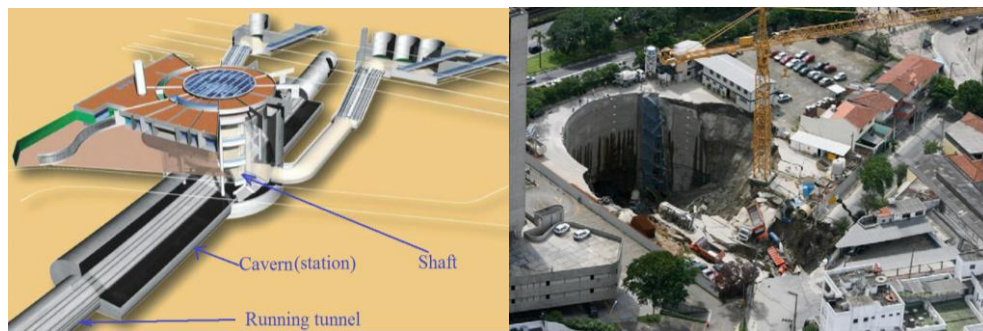
Figure 1 - (a) Artistic isometric view of the Pinheiros Station (after Barros et al. 2008), (b) collapse incident occurred on 12/Jan./2007, producing more than 20,000 t of failed mtl. During the bench excavation, very close of arriving to the shaft. The antidiаметrical failure surfaces extending around the shaft as is indicated by the arrow may be observed.
