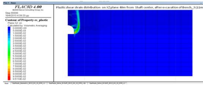
Figure 7 – (a) Final configuration of the shear band (localization of plastic shear) around the shaft and the cavern that finally collapses as a rigid body (one-quarter of the model). (b) Vertical section perpendicular to the cavern's longitudinal axis of the plastic showing the shear strain distribution.
