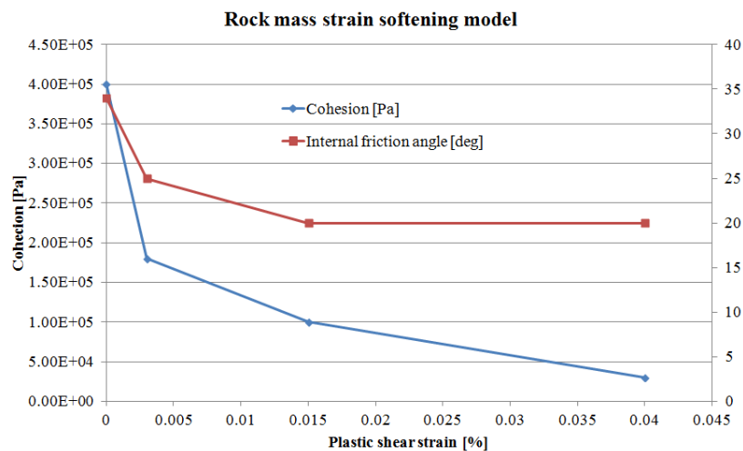
Figure 5 – Both c and \phi strain softening models.
