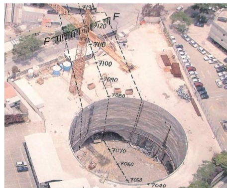
Figure 8 – (a) Displacement distribution after final excavation (b) IsoSurface of vertical displacement greater than 0.15 m (c) Aerial view of the Pinheiros Station shaft. The black curved arch at 20m depth down the shaft wall is the topheading of the station platform cavern. The shaft wall chainage at 7080 m and the rear discontinuity (FF) at chainage 7120 m, mark the approximate limits of the 40 m long station cavern collapse (Barton, 2009).
