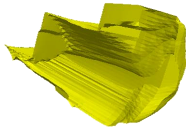
Figure 8 – (a) Displacement distribution after final excavation (b) IsoSurface of vertical displacement greater than 0.15 m (c) Aerial view of the Pinheiros Station shaft. The black curved arch at 20m depth down the shaft wall is the topheading of the station platform cavern. The shaft wall chainage at 7080 m and the rear discontinuity (FF) at chainage 7120 m, mark the approximate limits of the 40 m long station cavern collapse (Barton, 2009).
