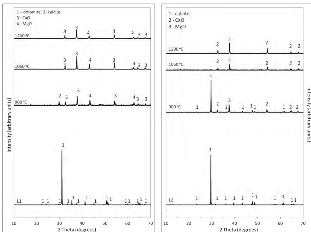
Figure 5 - XRD analyses of Q1 (left figure) and Q2 (right figure) samples for different calcination temperatures ( 900 , 1050 and 1200^\circ\text{C} ).
