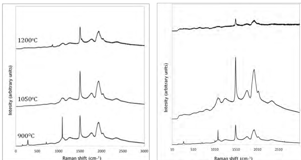
Figure 4 - Raman analyses for sample Q2 (calcite-rich), showing acquired spectra from its interior (left) and its surface (right).
