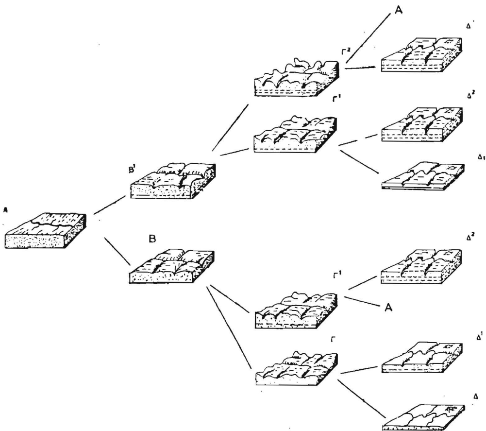
Σχ. 2. The Landform development of the geomorphological stages.
