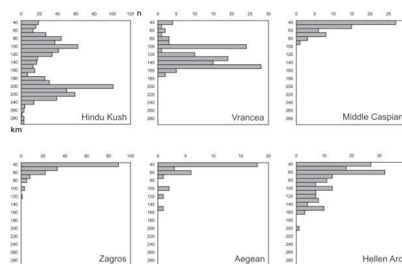
Fig. 1. Histograms of the number (n) of earthquakes with M_s \geq 5 in different depths (km) of the mantle seismic focal zones.
