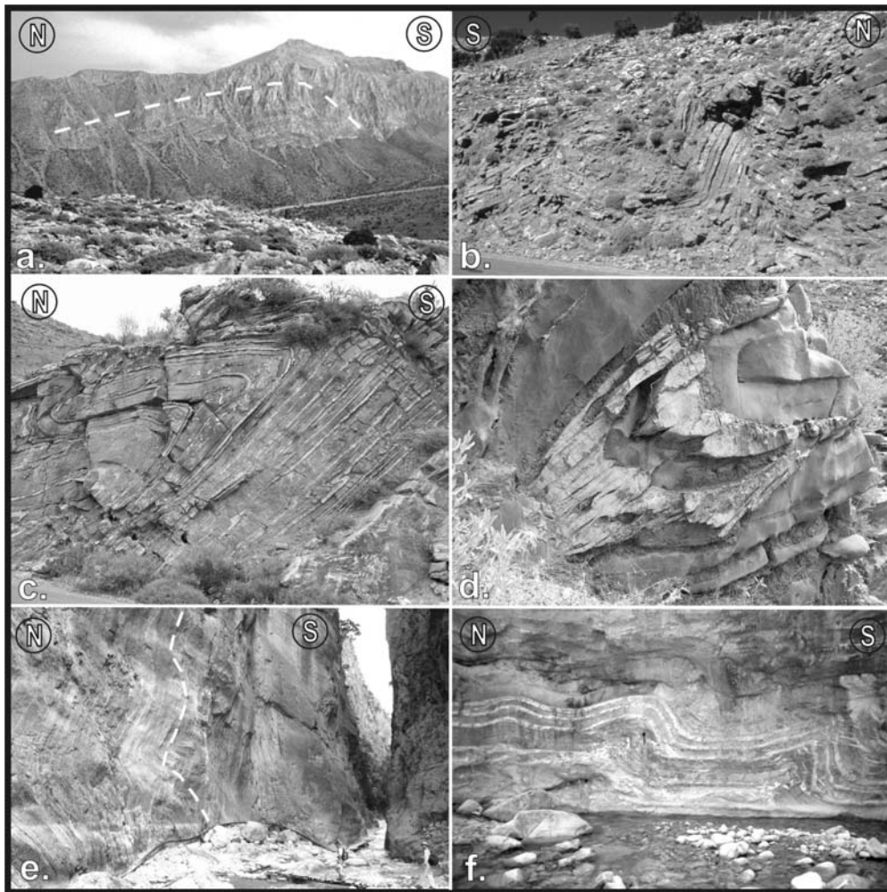
Photo 2. a. Large scale anticlinic structure (dashed line) at the face of Limnakaro fault, Lassithi mts (Fig. 1). b. Close, similar folding in Psiloritis Mountains (south of Anogia village), c. Recumbent, asymmetric fold in Vossakos area (see Fig. 3). Note thickening and buckle-folding at the inverted limb. d. Isoclinal folding and axial plane schistosity in Vossakos area (see Fig.3) illustrating a hinge zone thickened by flexural slip. e. Open angular folding at the inverted limb in Samaria gorge (Portes); axial plane approximately horizontal. f. Propagating deformation forming open-similar and asymmetric, drag folds in Samaria gorge. All pictures in platy marbles.
