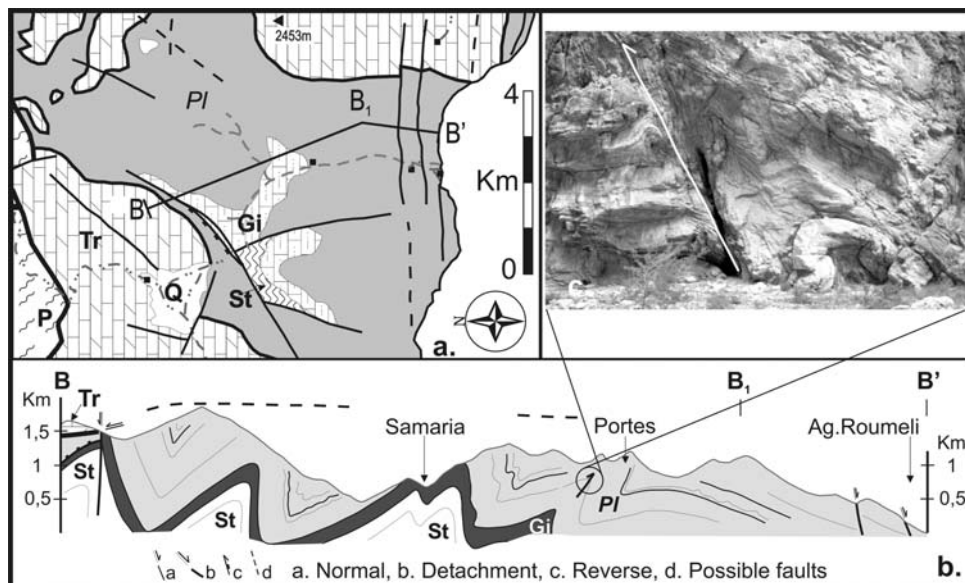
Figure 4. a. Geological map of Samaria area modified from Creutzburg et al. (1977) and Fytrolakis (1980). b. Cross section in Samaria area showing the folding of Plattenkalk nappe and major tectonic features (equal horizontal and vertical scales). c. Differential asymmetric folding in Samaria area inferred to be result of competence contrasts. Angular, isoclinal folding in thin-bedded marble; cylindrical, tight, folding in thick-bedded marble. Note thrust fault (white line) that developed during progressive deformation. Unlike the cross-section, the photo has north to the right. Symbols are: St, stromatolites; Gi, Gigilos beds; Pl, Platy marbles; P, Phyllite-quartzite nappe; Tr, Tripali nappe; Q, Quaternary sediments; double-dotted line, the main roads; gray-dashed line, Samaria stream.
