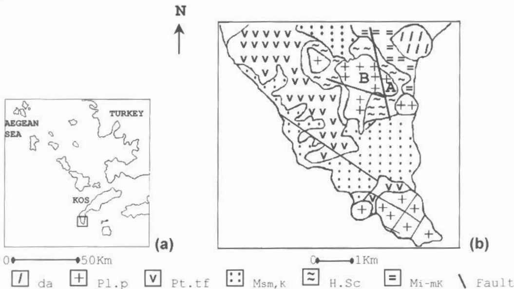
Figure 1. (a) Location of south Kefalos peninsula, Kos island. (b) Geological sketch map of South Kefalos peninsula, Kos island (Triantaphyllis, 1994) showing sample locations A and B.
