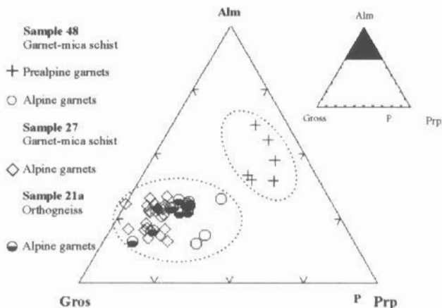
Figure 3: Ternary diagram (Almandine-Grossular-Pyropite) showing the compositional variation of garnets from garnet-mica schists (Samples 48, 27) and orthogneisses (Sample 21). In sample 48 the two generations of garnet, distinguished texturally, show, also, remarkable differences in their chemical composition.
