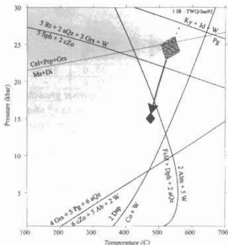
Figure 5: P-T diagram depicting reaction curves determined with the TWQ software program, for the Alpine HP metamorphic event. Real mineral compositions from garnet-mica schists and orthogneisses of Ios basement were used. Large diamond shows the approximate peak metamorphic conditions. Arrow shows the first stages of the decompression path.
