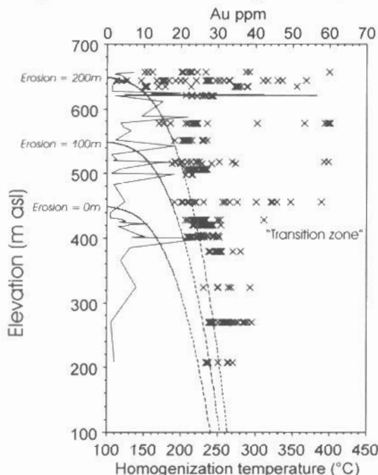
Figure 1: Relationships of fluid inclusion T_h versus elevation and Au assay for the Profitis Ilias deposit. Superimposed on the diagram are the dashed boiling curves calculated assuming an erosion of 0 m, 100 m and 200 m, since the mineralisation formation (see text for discussion).
