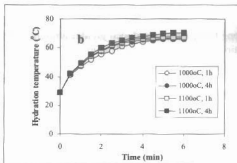
Figure 6. Hydration temperatures developed during slaking of the lime, a) 800 and 900 °C, b) 1000 and 1100 °C.
