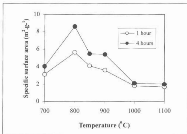
Figure 4. Evolution of specific surface area of the fired lime product as a function of firing temperature.
