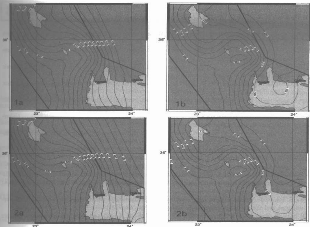
Fig 2: Hazard maps for models 1a, 1b, 2a, 2b respectively. The resulting curves show Peak Ground Acceleration calculated with Sadigh (1997) relationship for a return period of 475 years. The curve intervals are 10 gal
