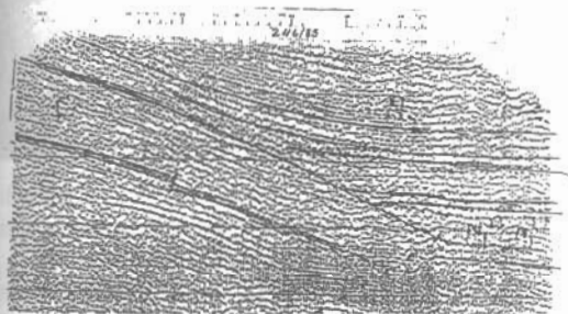
Fig. 6. Seismic line in southern part of Periadriatic Depression the unconformity between Miocene molasses and underlying folded flyschs and carbonatic deposits of Ionian zone is shown.
