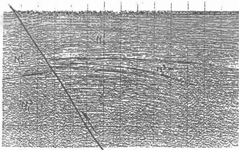
Fig. 10. Seismic line in Poverca region. The unconfornity between the Pliocene molasses is shown.
