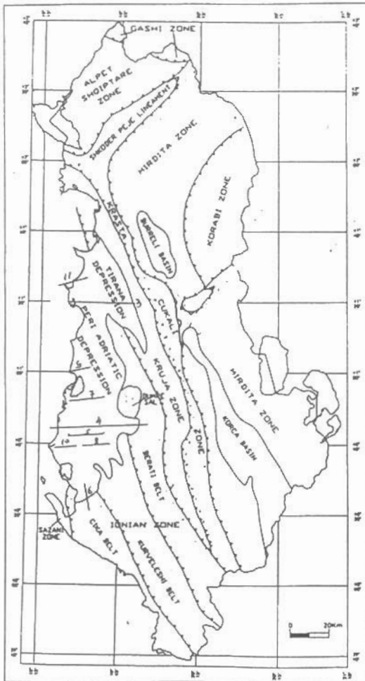
Fig.1. Tectonic map of Albania with the positions of seismic lines.
