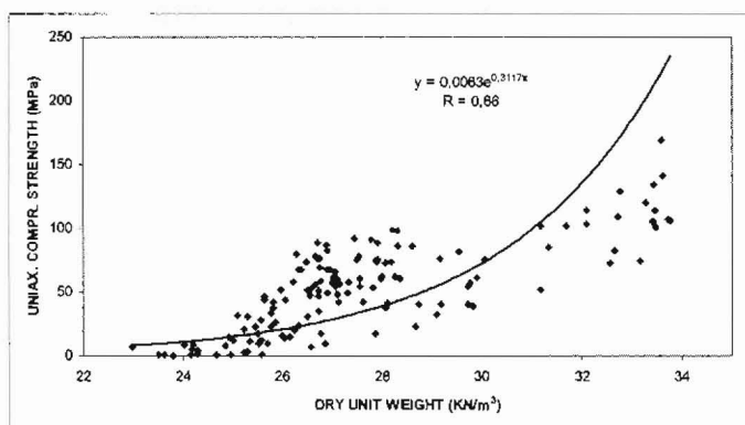
Figure 9 - UCS against Dry unit weight for the total number of ultrabasic samples
