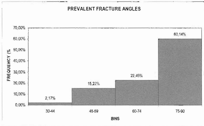
Figure 8 - Histogram of the prevalent fracture angles
