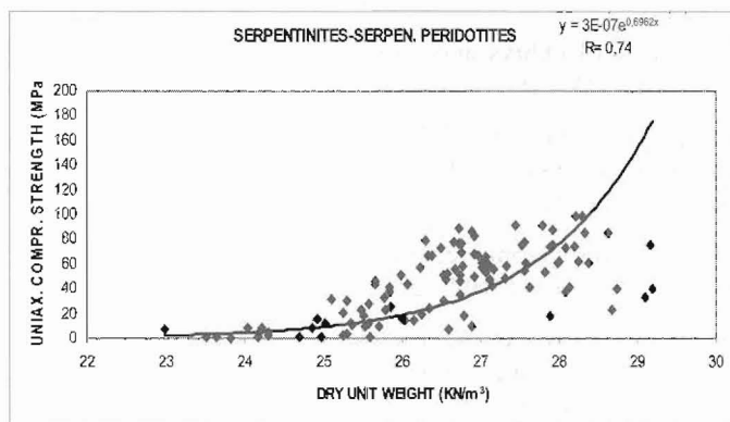
Figure 13 - UCS against Dry unit weight combining Serpentinised Peridotites and Serpentinites
