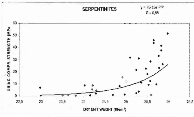
Figure 12 - UCS against Dry unit weight only for the Serpentinites
