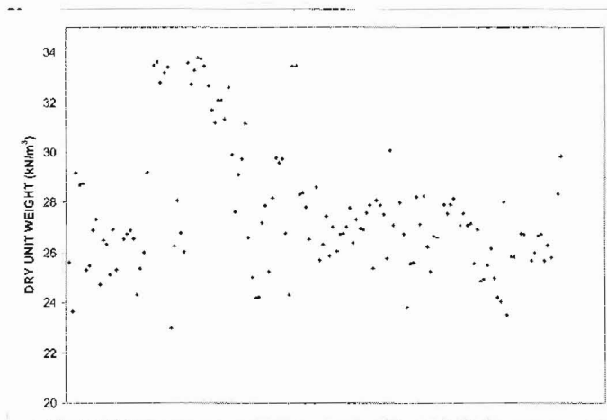
Figure 2 - Dry Unit weight values of the investigated ultrabasic samples
