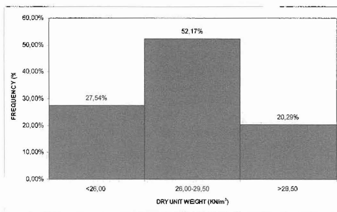
Figure 3 - Dry unit weight histogram
