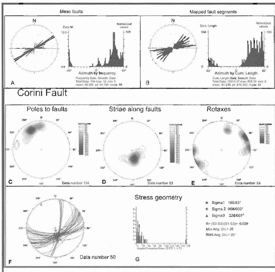
Figure 5 - Structural analysis of the Corini Fault. The data comprise 134 measurements of strike and dip angle and 53 measurements of rake angle on the fault plane. North is marked by “N”. A) Data portrayed on rose diagrams: Strike of fault planes and histogram of fault plane orientations (azimuth). B) Histogram of fault segment length vs. fault segment azimuth showing that NE segments are more important in accumulating fault length. C) D) E) Data are portrayed on lower hemisphere equal-area projections (Stereonet). Stereonets portray all data as contoured poles to the strike and dip of planes and trend and plunge of lines. The percent data at the contoured point maximum is indicated to the right of each stereonet. The number of points in the data sets is indicated in the lower right of each diagram. F) & G) Paleostress analysis. Stress axis terminology is as follows: sigma 1 denotes trend and plunge of maximum principal stress, sigma 2 of intermediate stress and sigma 3 of least stress, respectively
