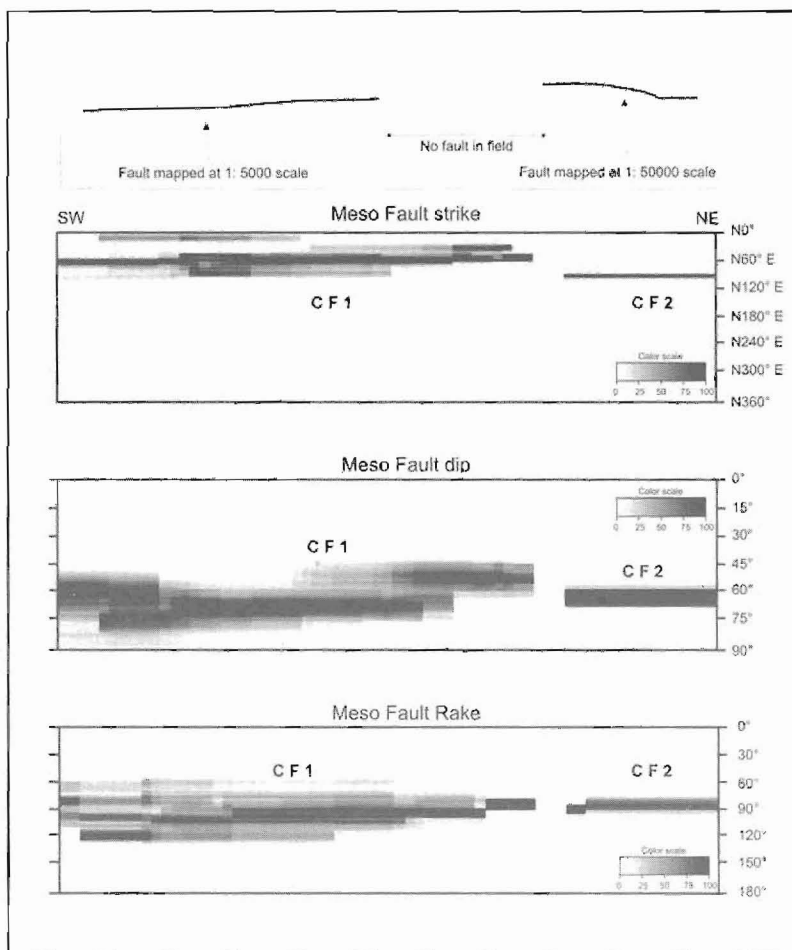
Figure 6 - Transect Analysis of the Corini Fault. Line brightness is proportional to the volume of data collected in the field. It can be seen that segment CF2 strikes N100°E, dips 60°-70° south and rake is almost 90°, i.e. motion is pure dip-slip. However, the rake along the segment CF1 is mostly > 90° indicating right-lateral movement
