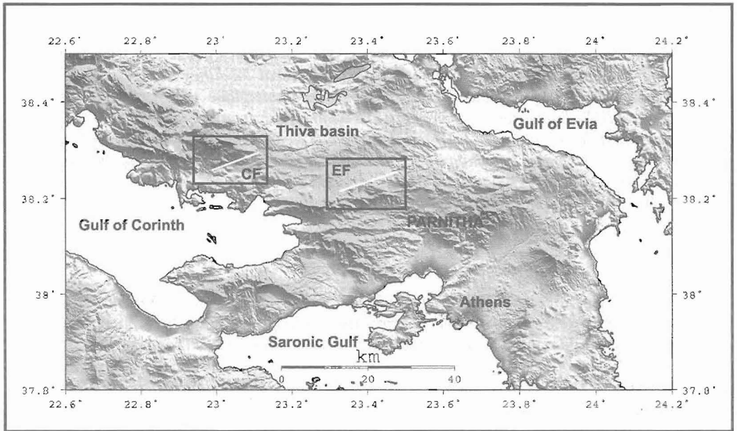
Figure 1 - Shaded relief map of Attica and Viotia regions in central Greece. Illumination is from the north-east. Black rectangles indicate locations of Corini Fault (CF) and Erithres Fault (EF), respectively. Area of rectangle CF is shown in Figure 2, below. Thin white lines indicate linear traces of active faults. Elevation data were provided by the SRTM mission
