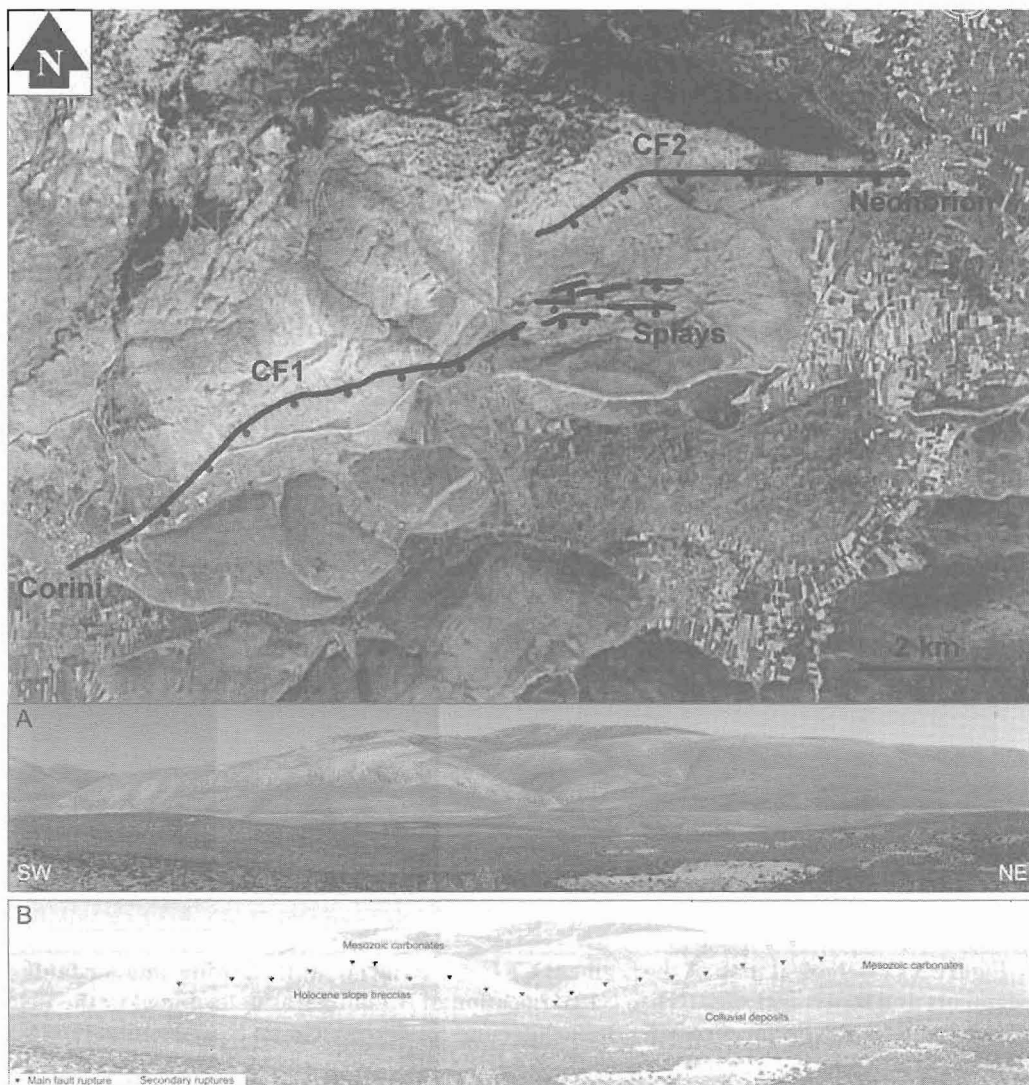
Figure 2 - Satellite image and corresponding field photograph of the Corini normal fault in south-west Viotia region, central Greece. Top: Landsat image with superimposed traces of active faults. Middle: Original picture, Bottom: main fault plane is indicated by a series of black triangles. Secondary planes are shown by the alignment of white triangles. The main rock types are also indicated. The highest altitude of the fault plane is approximately 480 m. View to the Northwest. Photograph taken 14 June 2006
