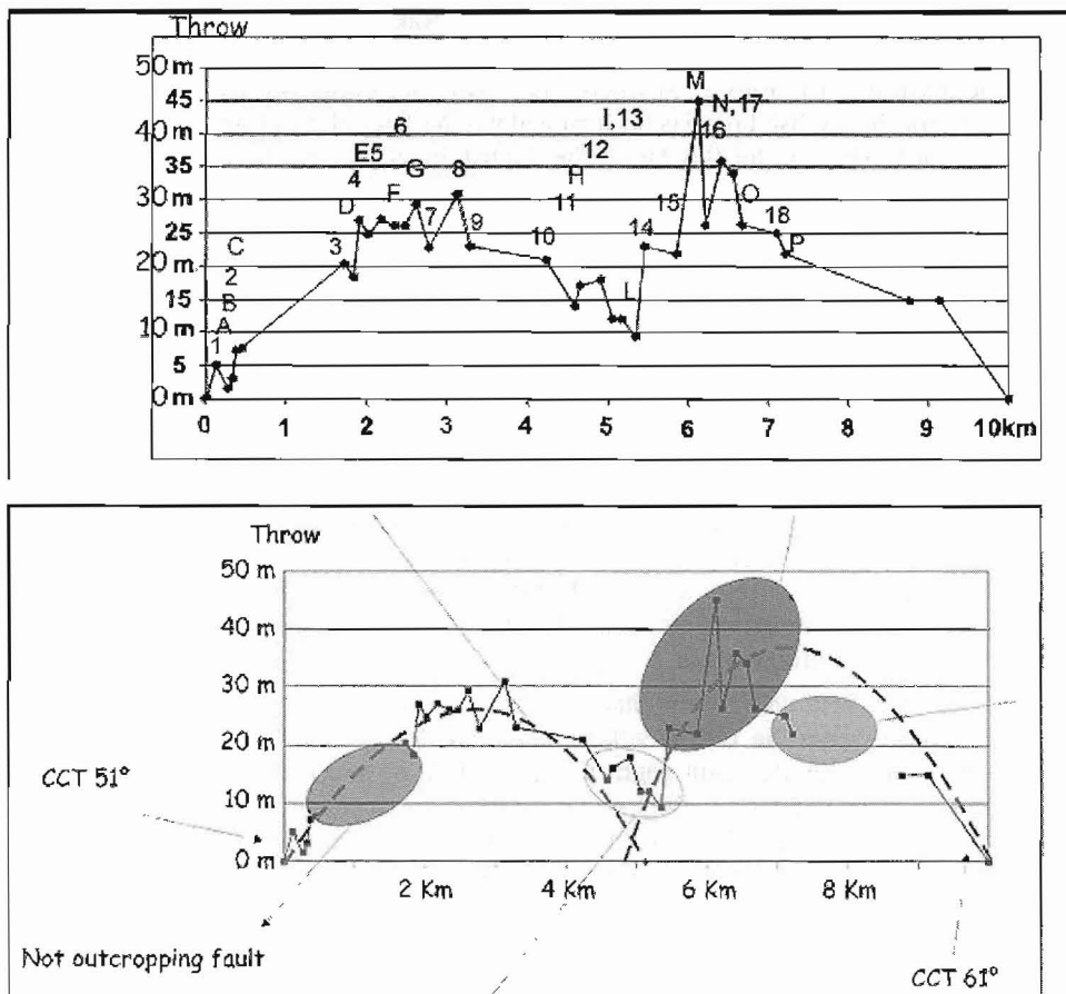
Figure 8 - (Top) Displacement-Length diagrams for the Corini Fault – segment CF1. Data points (black boxes with labels) originate from morphological profiles of Figure 7. We suggest that morphological offset is representative of fault displacement because of similar bedrock lithology and fault dip direction along strike. We observe that the profile does not fit the ideal, elliptical shape but shows two maxima at 2-3 km and 6-7 km, respectively. (Bottom) Sketch for interpretation of top graph. The profile can be split into two parts, each one with almost similar bell-shaped profile. The area between 4 and 6 km shows low throw values which suggest a linkage of two CF1 proto-segments
