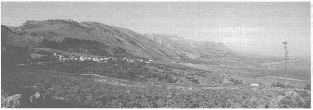
Figure 2 – The Sfakia fault expressed as a steep south-facing, morphological discontinuity striking E-W and separating a narrow coastal zone from the eastern foothills of the Lefka Ori massif. View to the east
